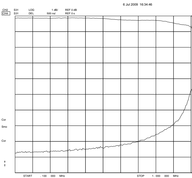
Passband Response (1 dB/div & 500 nsec/div)
