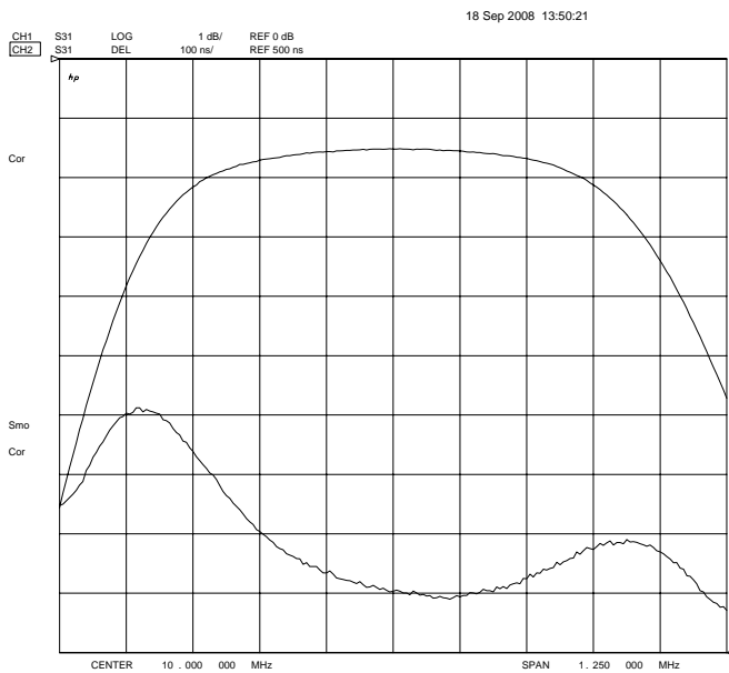
Passband Amplitude & Group Delay (1 dB/div & 100 nsec/div)
