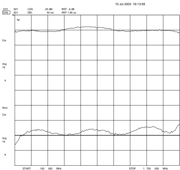
Passband Amplitude & Group Delay (0.25 dB/div & 50 nsec/div) 100 KHz to 1.75 MHz
