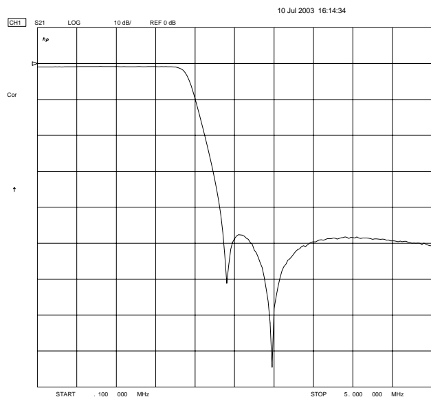
Overall Response (10 dB/div) 100 KHz to 5 MHz
