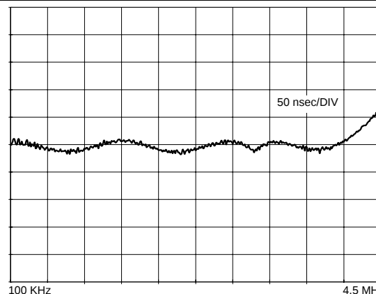
Group Delay Deviation from Standard
