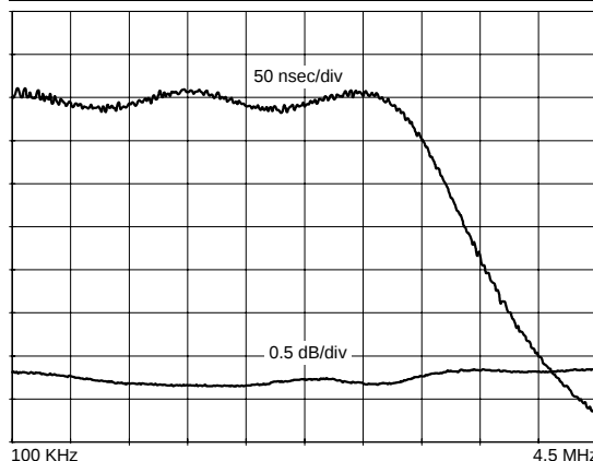
Passband Amplitude & Group Delay
