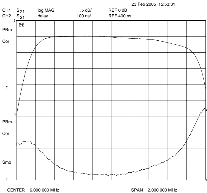
Passband Amplitude & Group Delay (0.5 dB/div and 100 nsec/div)
