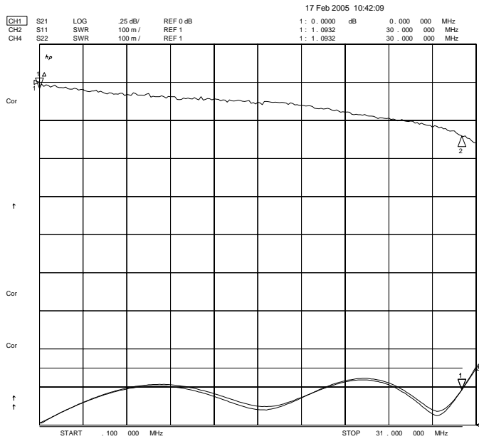
Passband Amplitude & VSWR (0.25 dB/div and 0.1/div)
