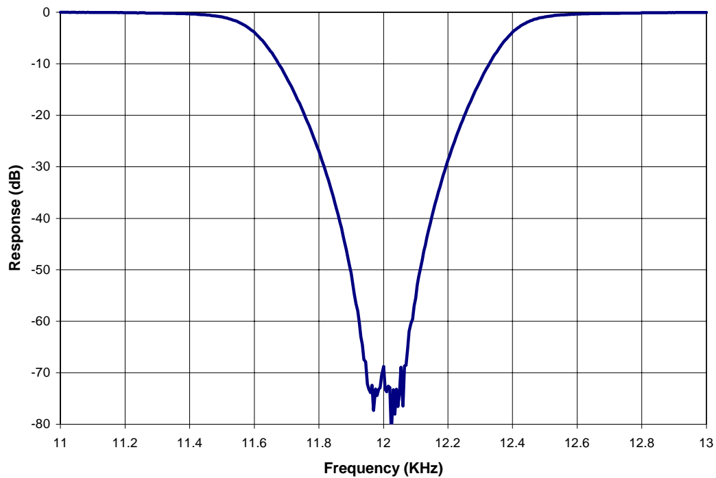
Overall Response (10 dB/div)
