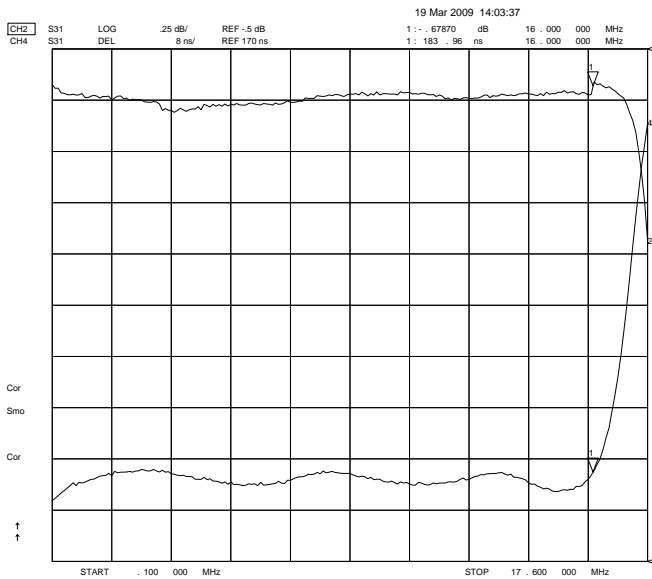
Passband Response (0.25 dB/div & 10 nsec/div)
