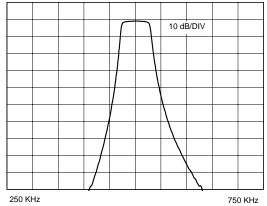
Overall Amplitude
