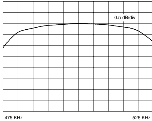
Passband Amplitude
